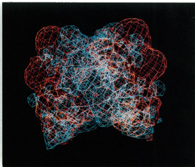
(3f) A. p. piscivorus dimer 0 degrees - 1.0 kT - 0 calcium ions.
