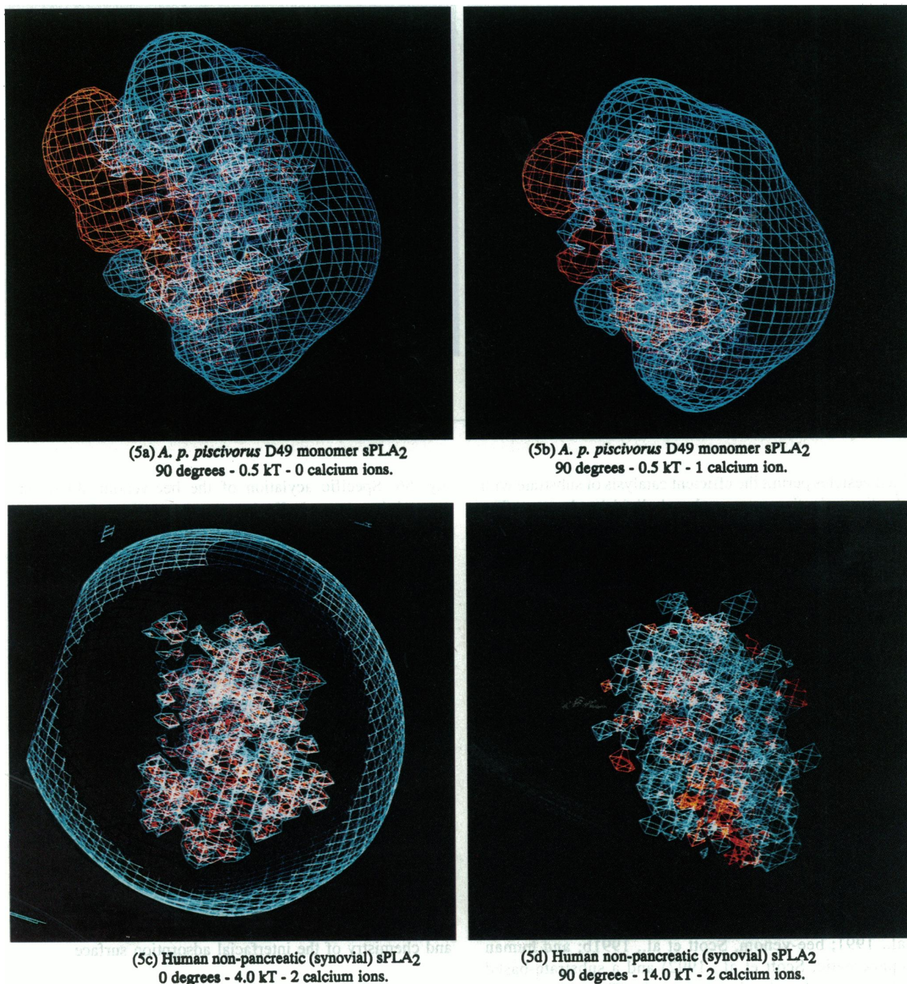
FIGURE 5 Electrostatic potentials calculated from the coordinates of crystalline phospholipases A 2 : category III. Figures depict the electrical potentials of one or both standard orientations (0°/90°). An electrostatic potential of 1 kT/e (where k is the Boltzmann constant and T is the Kelvin temperature) is equal to 25 mV at 300 Kelvin. The contour levels of the maps were chosen to provide the maximal pictorial information possible about the respective electrostatic potential magnitudes and orientations. A contour level of 1 kT means that an atom of one unit of positive charge, sitting at a point on the contour grid, would have an interaction energy of +1 kT (approximately +0.6 kcal/mole at 300 Kelvin) with the electrostatic potential at that point. No correction was made for the over-estimation of electrostatic charge potentials by the linear Poisson-Boltzmann equation for c and d . Blue is used to indicate positive potentials, and red is used to indicate negative potentials. a. A. p. piscivorus sPLA 2 (49 monomer): 90 degrees—0.5 kT—0 calcium ions. b. A. p. piscivorus sPLA 2 (D49 monomer): 90 degrees—0.5 kT—1 calcium ion. c. Human nonpancreatic (synovial) sPLA 2 : 0 degrees—4.0 kT—2 calcium ions. d. Human nonpancreatic (synovial) sPLA 2 : 90 degrees—14.0 kT—2 calcium ions. e. Porcine pancreatic sPLA 2 : 90 degrees—1.0 kT—0 calcium ions. f. Porcine pancreatic sPLA 2 : 90 degrees—1.0 kT—2 calcium ions.
